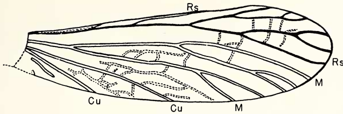
Fig. 2. Drawing of visible veins and reticulations of holotype forewing of Cretatermes carpenteri , new genus, new species.
